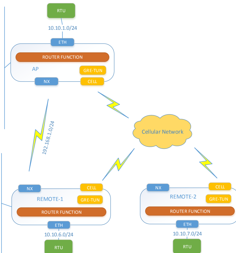
Figure 3-227. MCR to MCR NX+CELL redundant network (layer-3) setup using routing
