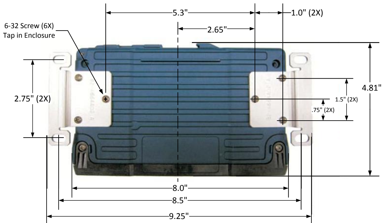
Figure 2-7. MCR Flat Mounting Bracket Dimensions
